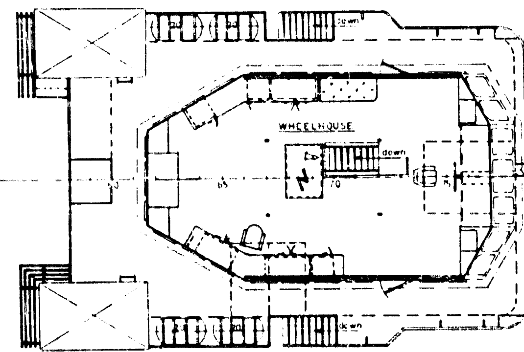
Bridge Deck
