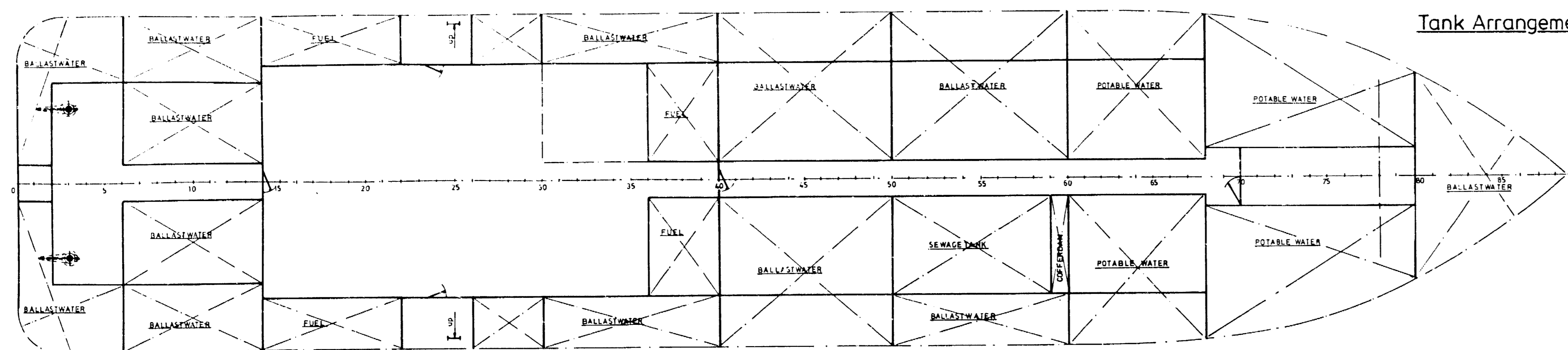
Tank Arrangement
